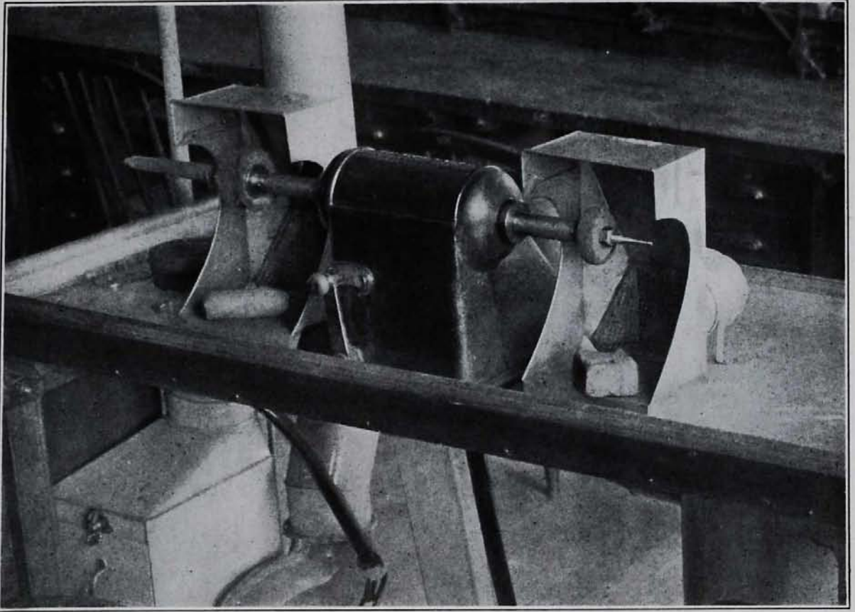
FIGURE 172 Polishing Head showing dust collector
