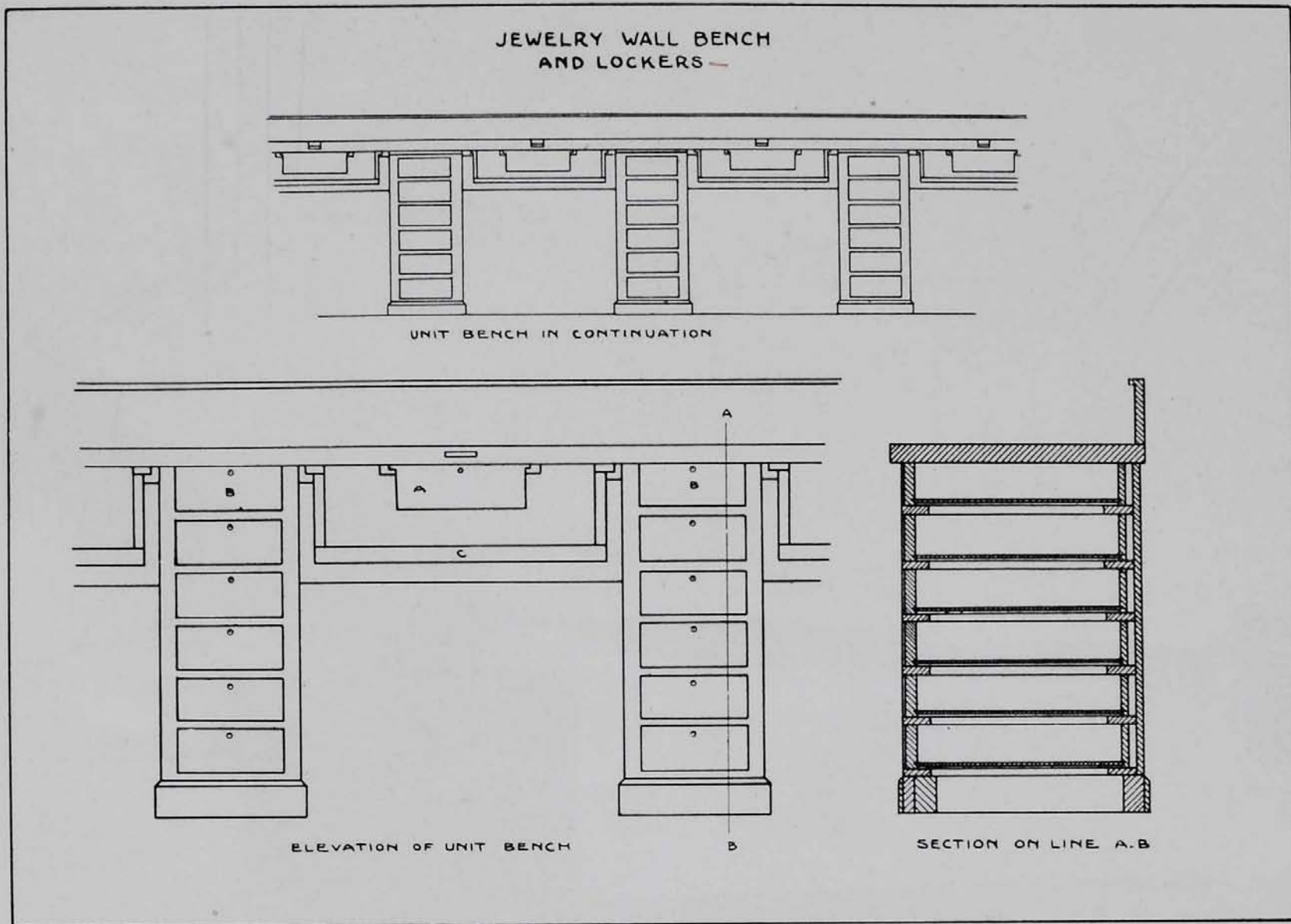
Elevation of Bench shown on Page 236, Figure 154
