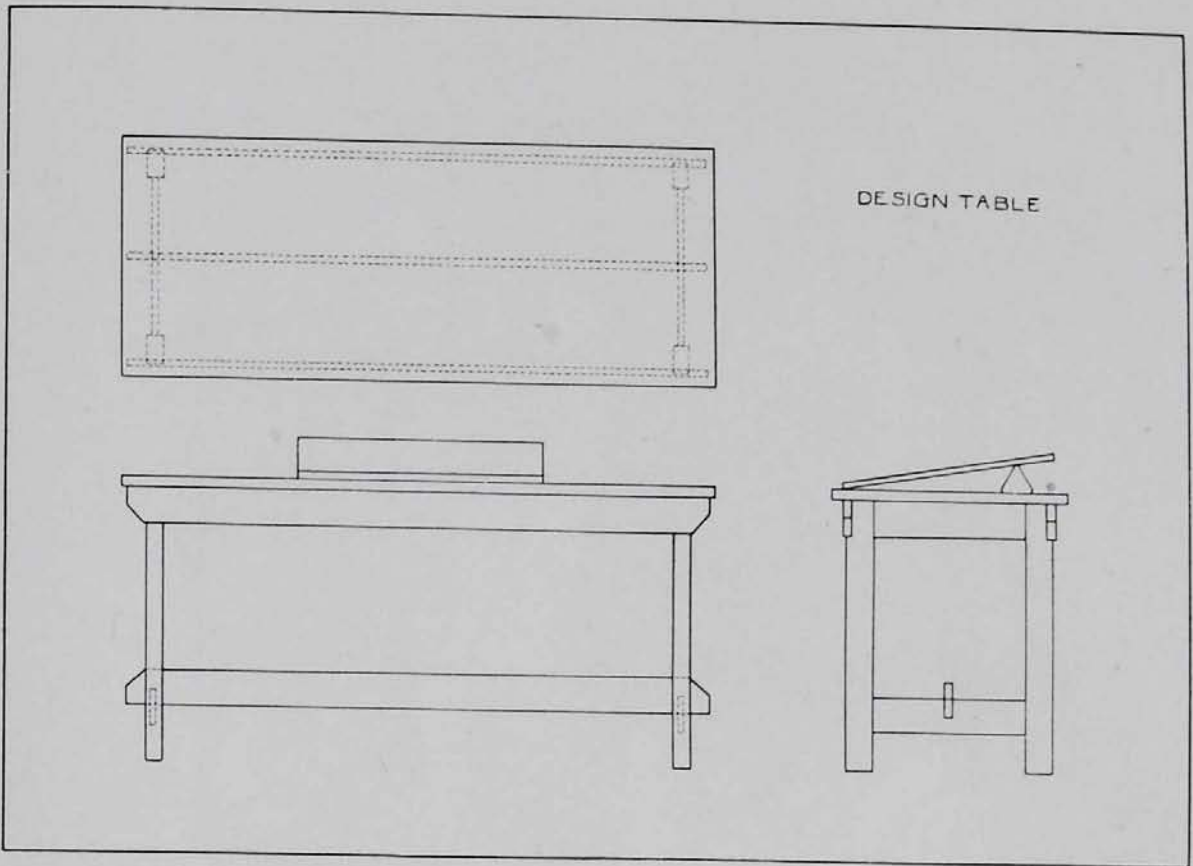
FIGURE 168 An inexpensive table for work in Design
