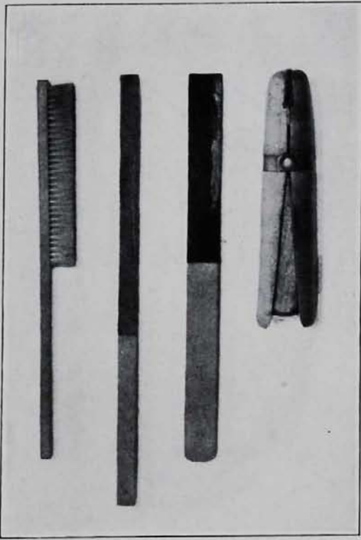
FIGURE 162 Bench Brush Polishing Sticks Ring Clamp
