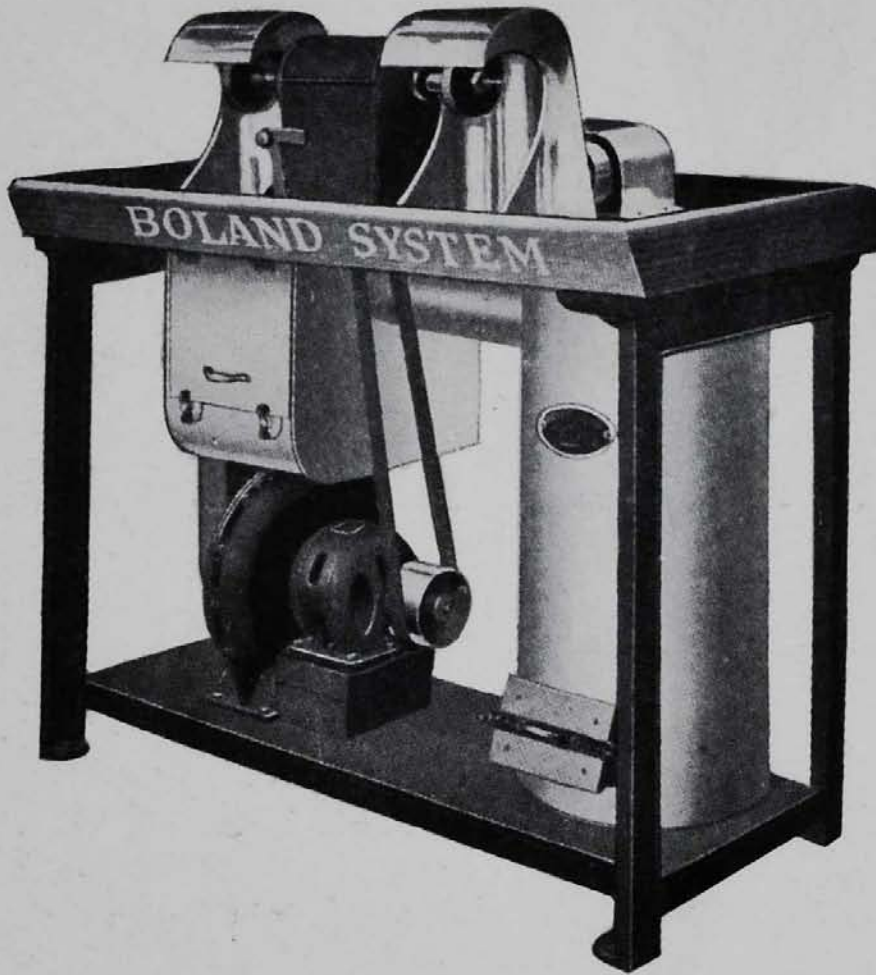
FIGURE 170 Polishing Bench
