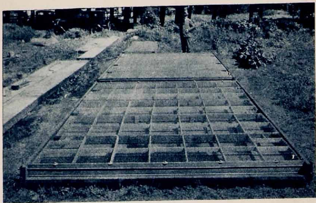
Fig. 7. Two 1/200 acre basins joined together as one unit of 1/100 acre. Seedbed consists of ten frames, each 4 feet wide, 12 feet long, supported within the basin.
