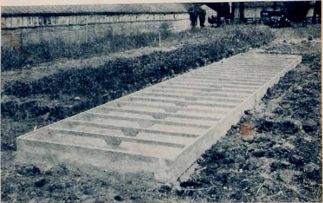
Fig. 2. First concrete basin, 6 feet wide, 36 feet long, six inches deep or 1/220 acre inside measurement. The concrete cross-bars to hold wire netting have since been discarded.
