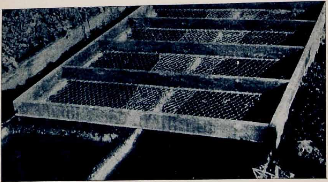
Fig. 6. Seedbed frame constructed to rest on top of the basin. This is a better arrangement than to have the seedbed mounted within the basin.
