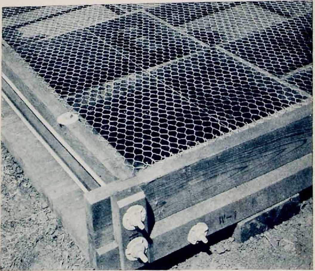
Fig. 4. Section of a wooden basin showing the wire netting in place and the ends joined together by means of tie rods and croze. The basin is of two-inch planking, 18 feet long. The planks are straight-edged. No nails are used. Assembling such a basin consists simply of placing the pieces, inserting twelve tie rods in holes bored for the purpose, and drawing the pieces together. This basin is more substantial than necessary.
