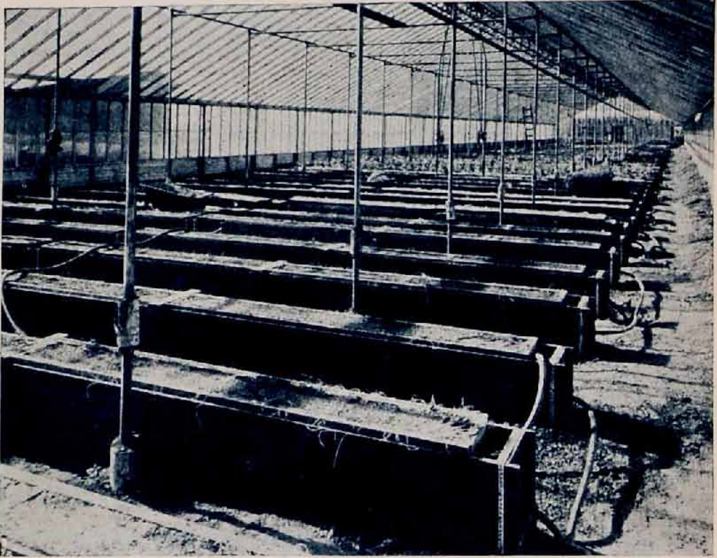
Fig. 50. The first commercial hydroponicum built of redwood. Basins one foot wide and 36 feet long have been in use five years. The solutions circulate through the basins.
