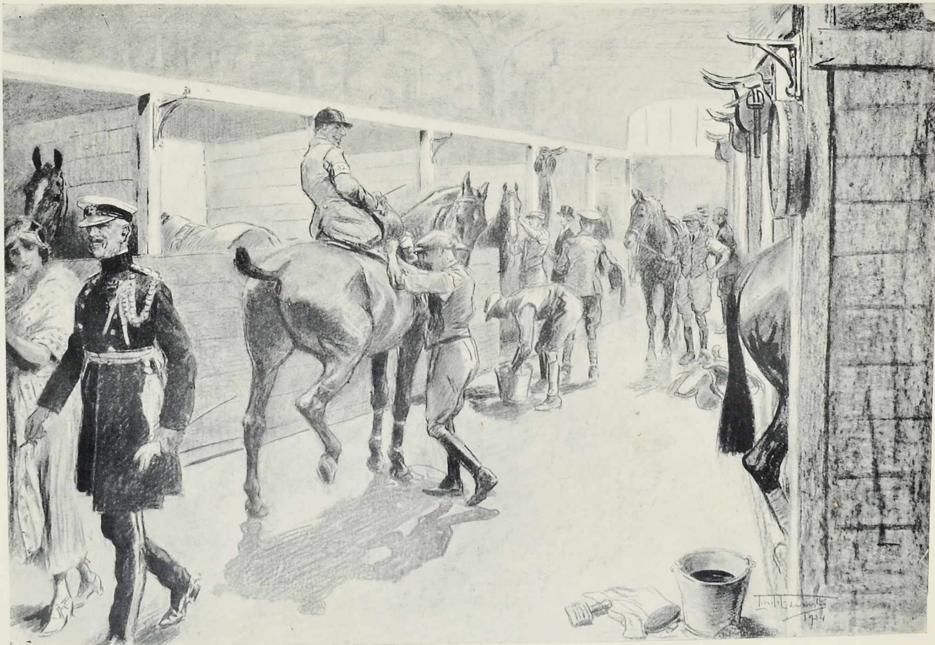
CARELESS GIRTHING.
