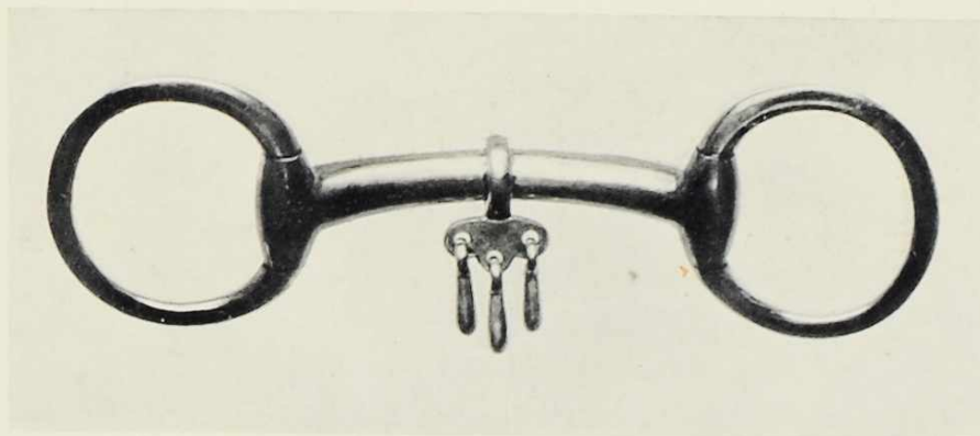
FIG. 6. A recently designed breaking bit, suitable for a very young horse. For a light mouth it is preferable to Fig. 14, and a further improvement might be to cover it with vulcanite.
