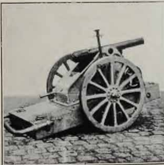
NEW GERMAN BOMB-GUN.
