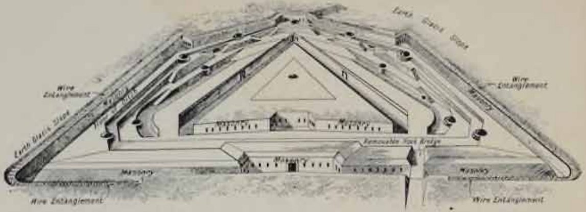
PENTAGONAL BRIALMONT FORT.
